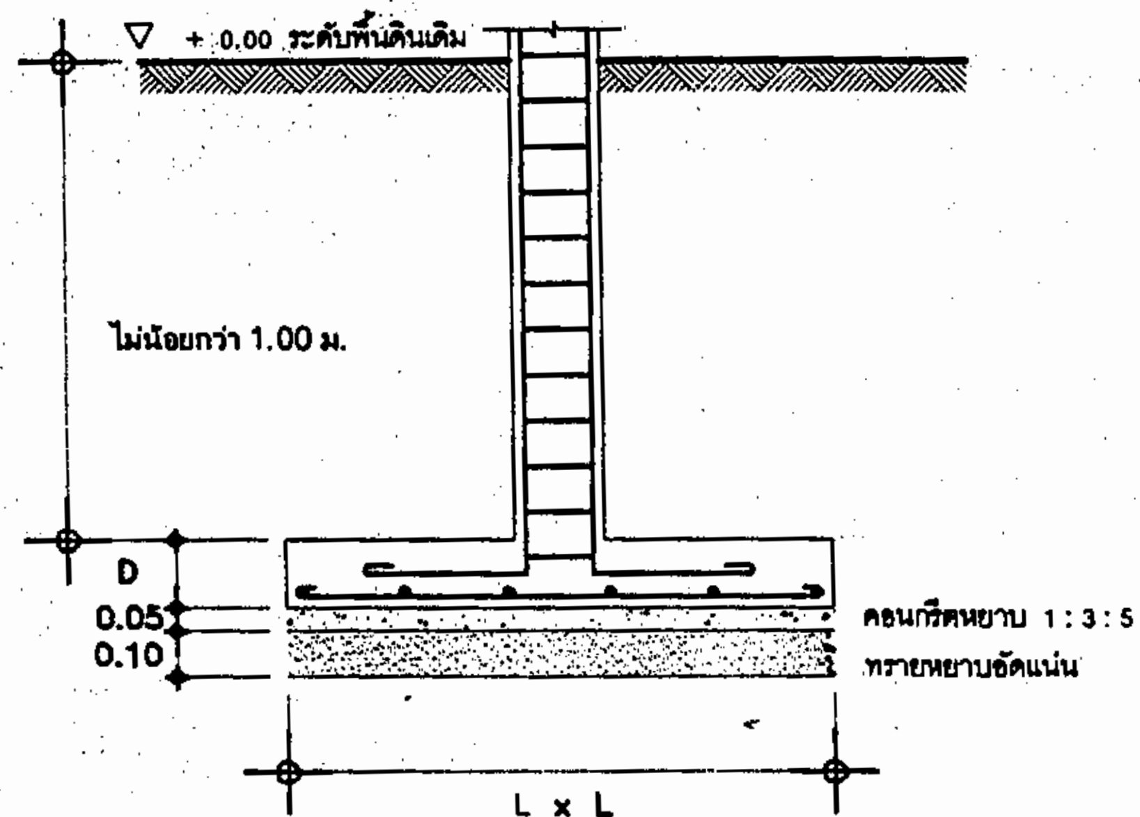
F SECTION
